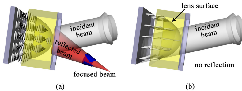
Fig. 1. Operating principle of the switchable reflective lens of the CLC. (a) reflected beam with circular polarization coinciding with the helix of the CLC is focused in the planar alignment of the CLC. (b) No reflection occurs at the homeotropic alignment under an applied voltage.
