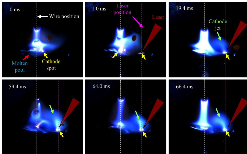
FIG. 7. Stabilization of the cathode spot location by laser irradiation (laser power: 1500 W, offset: 6 mm).
