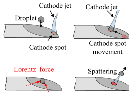
FIG. 5. Spatter generation mechanism in Ti GMA-WAAM.
