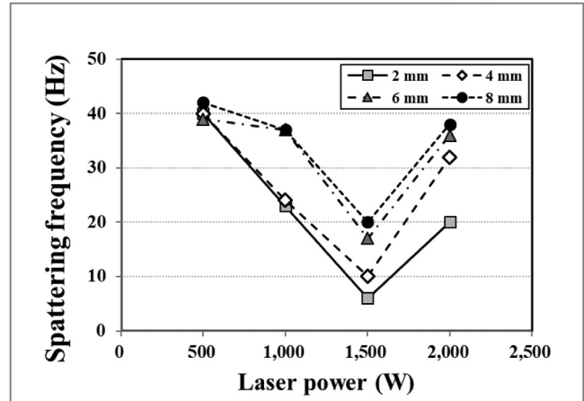
FIG. 11. Effect of laser power on spatter generation. The number of spatters was counted during a 1.0 s interval.
