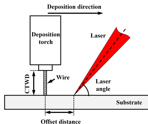
FIG. 1. Schematic diagram of torch and laser beam arrangement.
