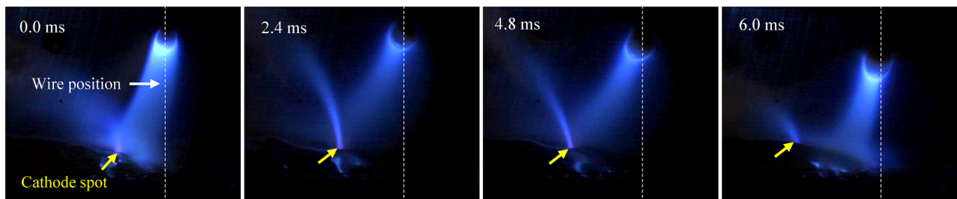
FIG. 17. Arc wandering in an oxide prelaying test.
