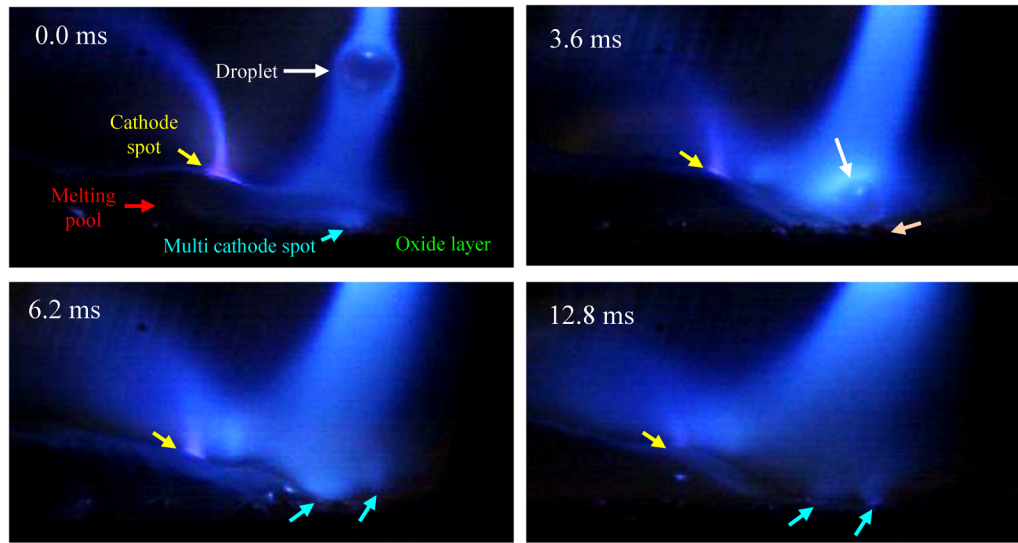
FIG. 16. Multiple cathode spots from oxides.
