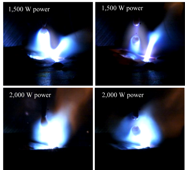
FIG. 12. Cathode jet and plasma behavior according to the laser power at an offset distance of 2 mm.
