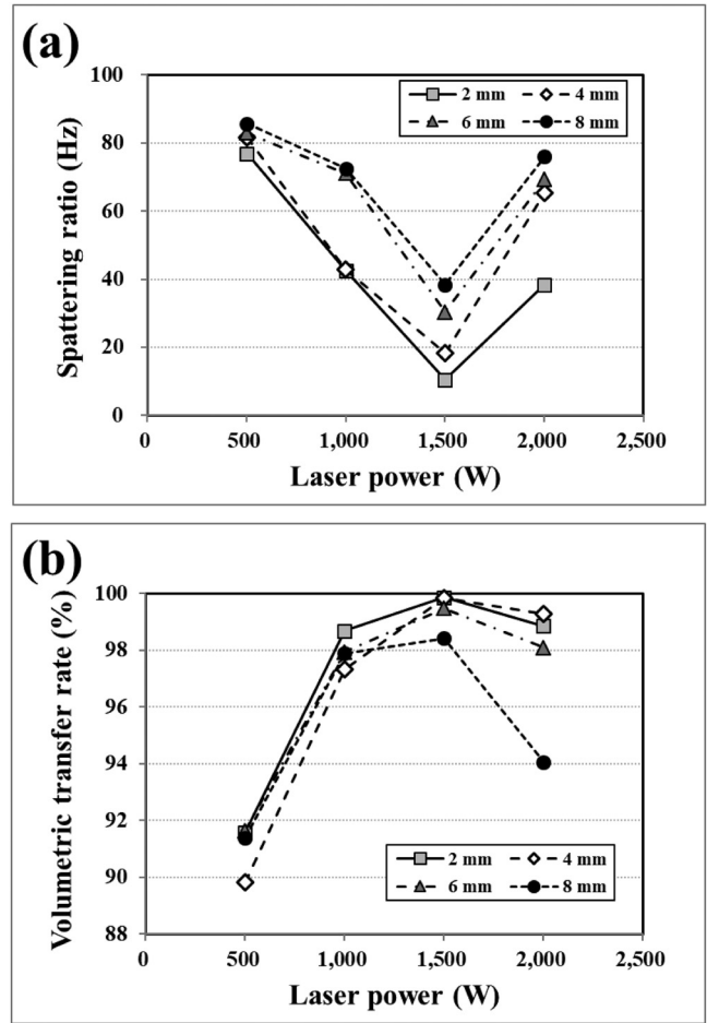
FIG. 14. Calculated (a) spattering ratio and (b) volumetric transfer rate.
