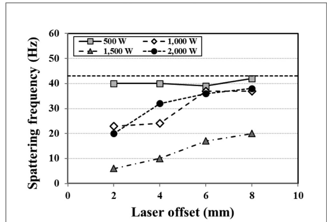
FIG. 8. Effect of laser offset on spatter generation.
