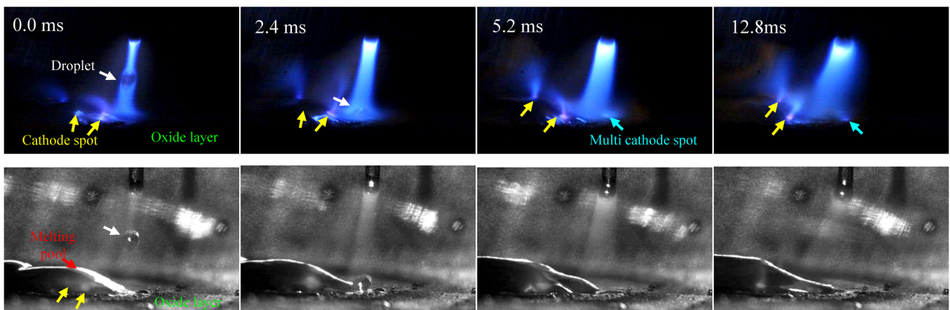
FIG. 15. Cathode spot behavior in an oxide prelaying test.
