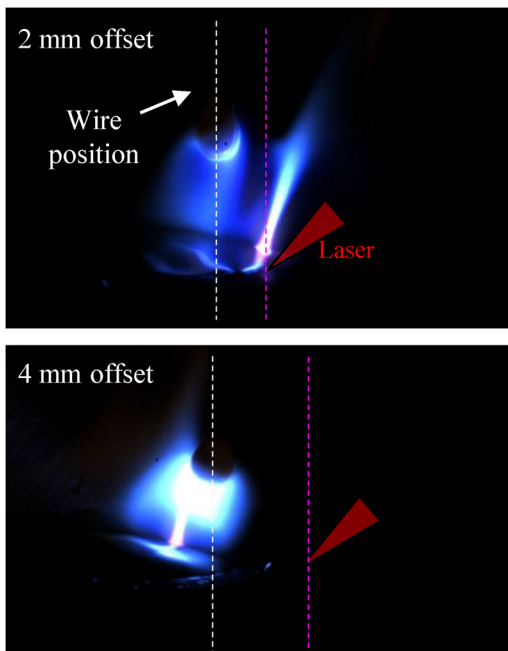
FIG. 10. Cathode jet behavior according to the laser offset at a laser power of 500 W.
