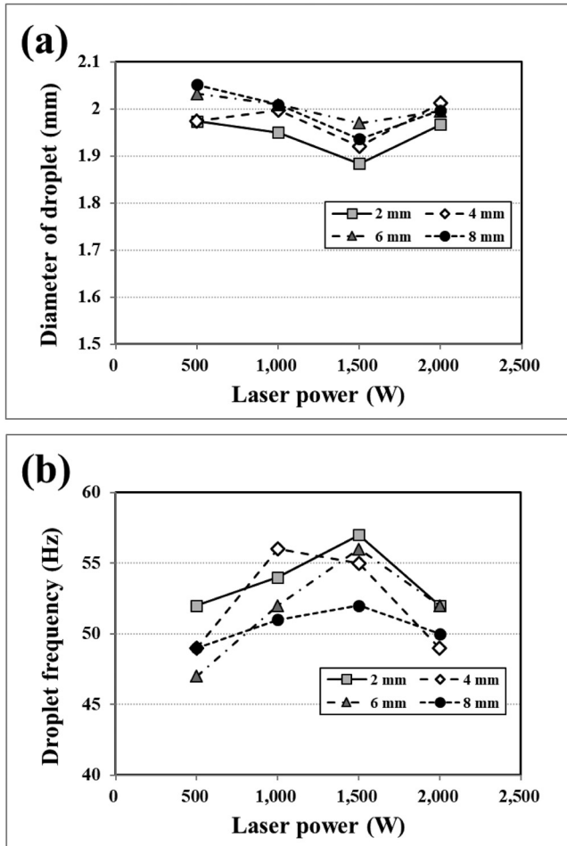
FIG. 13. Measured (a) diameter and (b) frequency of free flight droplet.
