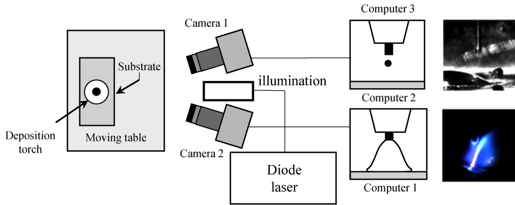
FIG. 3. Schematic of high-speed photography.
