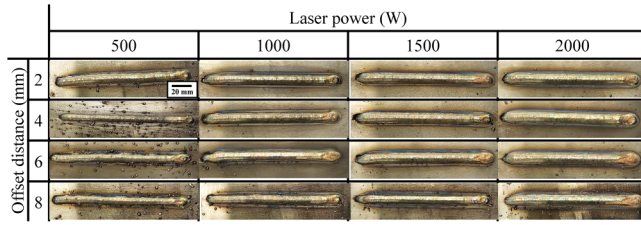
FIG. 6. Effects of the offset distance and laser power on spatter generation.
