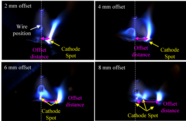
FIG. 9. Cathode jet behavior according to the laser offset at a laser power of 1500 W.
