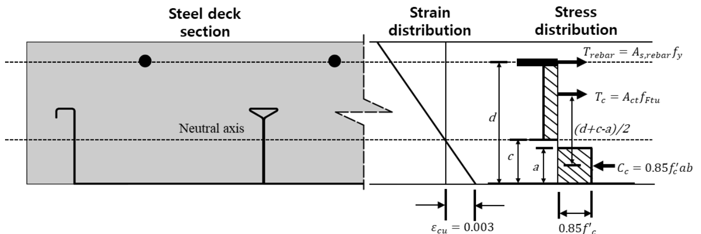
Figure 14. Strain and stress distributions (negative moment).
