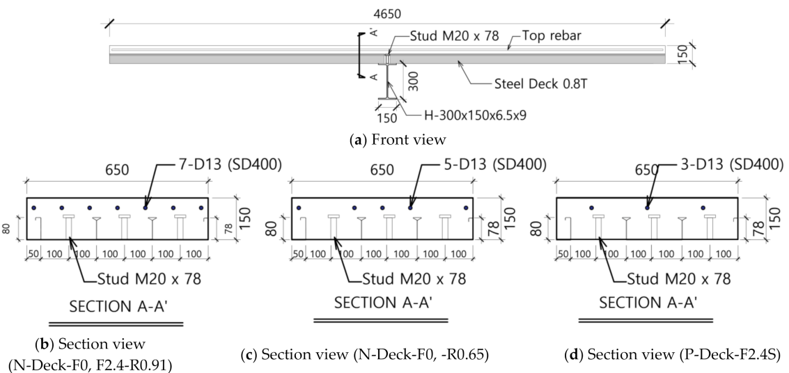
Figure 6. Negative moment test specimen details (unit: mm).
