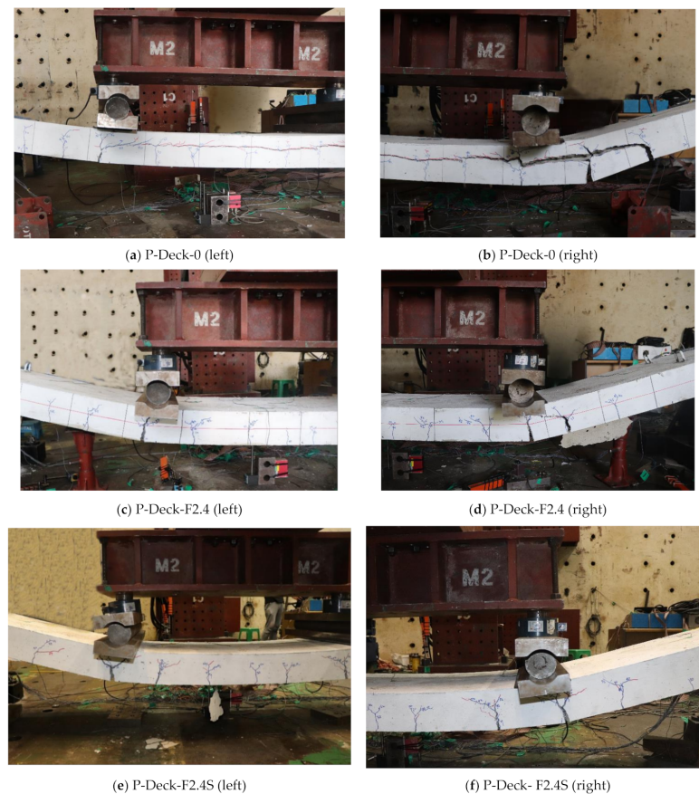
Figure 8. Crack and failure patterns (positive moment test specimens).
