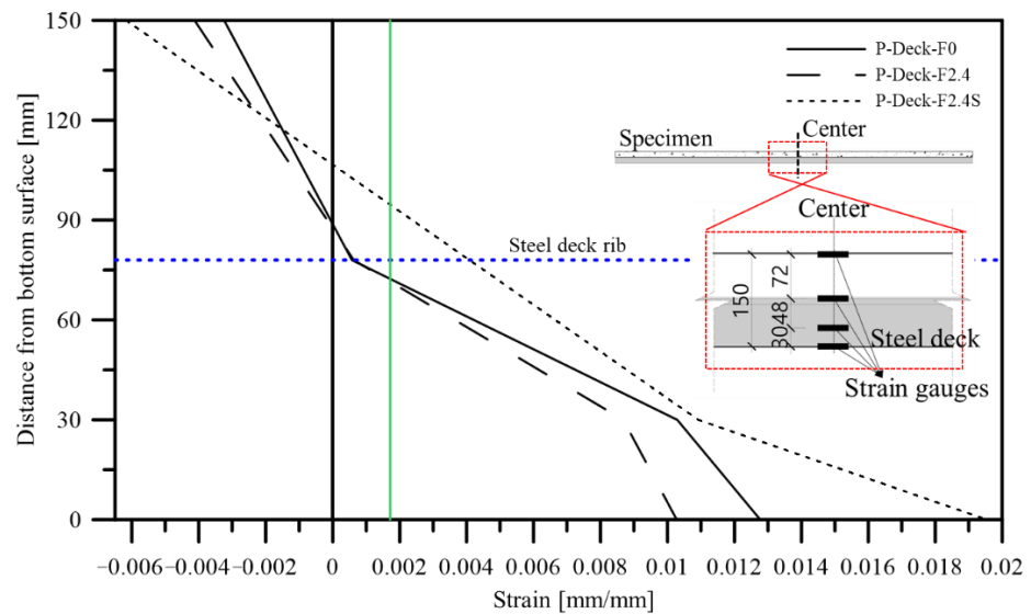
Figure 11. Strain distribution at the center of specimens (unit: mm).
