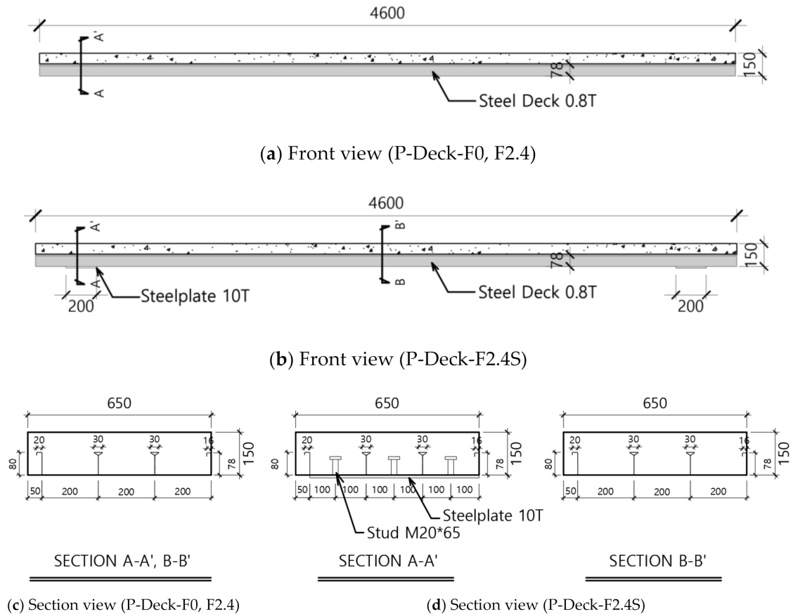
Figure 5. Positive moment test specimen details (unit: mm).
