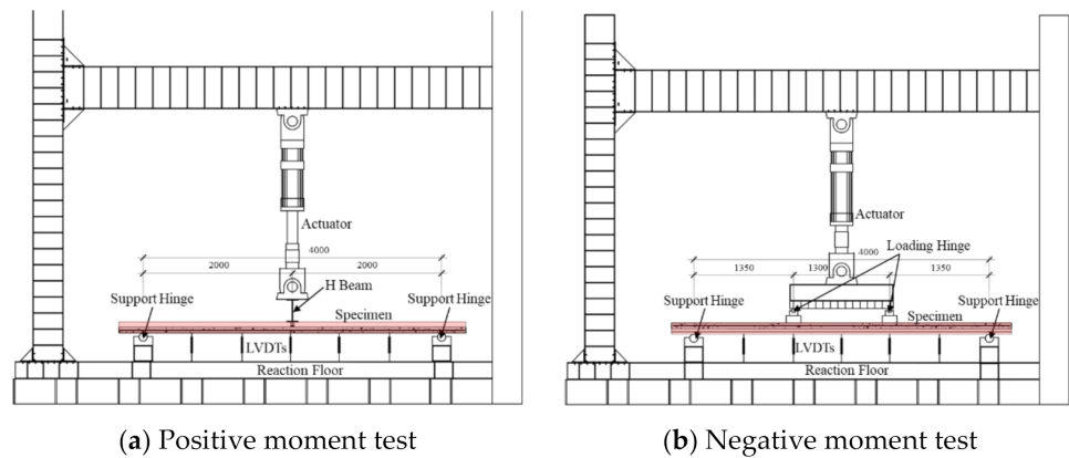
Figure 7. Test setup (unit: mm).
