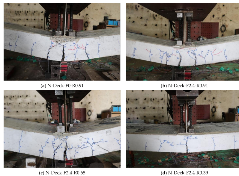
Figure 9. Crack and failure patterns (negative moment test specimens).
