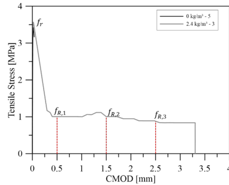
Figure 3. Load–crack mouth opening displacement (CMOD) relationship.
