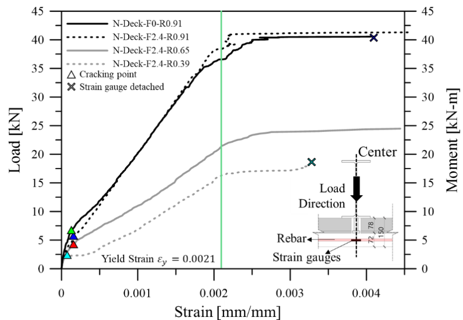
Figure 12. Load–strain relationship (negative moment test specimens; unit: mm).
