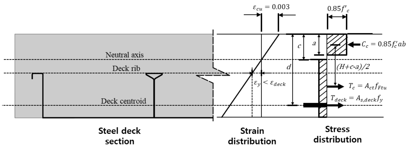
Figure 13. Strain and stress distributions (positive moment).
