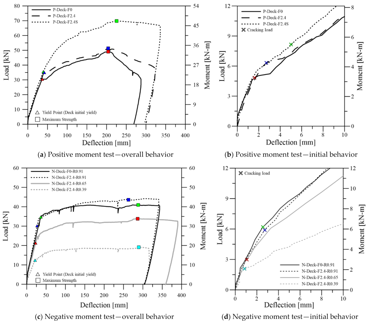
Figure 10. Load–displacement relationships.
