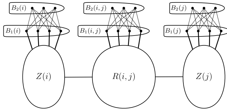
Fig. 5. A part of the graph G' , where 1 \leq i < j \leq k and d = 4 .
