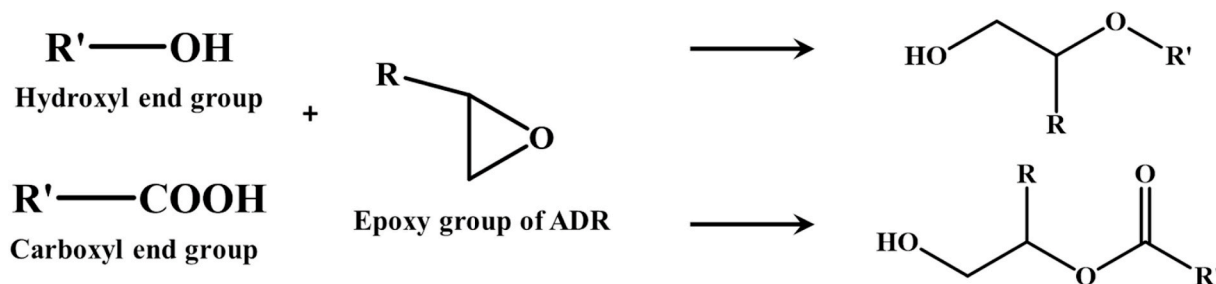
Scheme 2. Compatibilization reaction of ADR [49].
