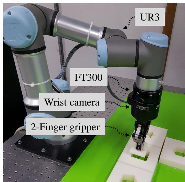
Figure 4. Experimental setup for peg-in-hole task.
