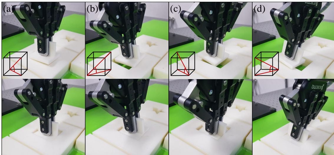
Figure 6. Four peg directions of a human demonstration of the “hole search” and “peg insertion” motor skills of the peg-in-hole task: (a) 30°; (b) 120°; (c) 210°; and (d) 300°. The upper and lower rows illustrate the motions of “hole search” and “peg insertion”, respectively. In the upper low, the black boxes (holes) and red lines (pegs) indicate relative postures.
