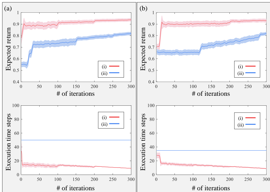
Figure 8. Performance with respect to two reward functions and the original PoWER and iPoWER algorithm in the peg-in-hole task for the motor skills: (a) “hole search”; and (b) “peg insertion”. The upper and lower rows illustrate the return values and number of execution time steps, respectively. The red lines indicate the results using the iPoWER algorithm, and the blue lines indicate the results using the original PoWER algorithm.
