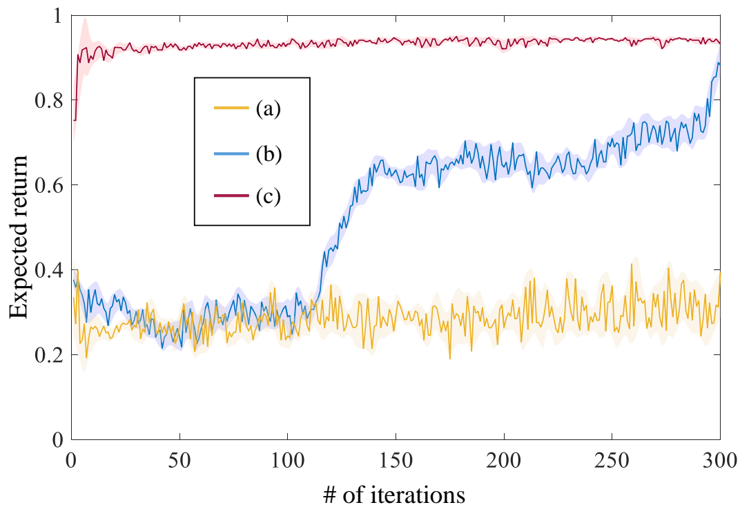
Figure 9. Expected returns of policy parameters with respect to number of iterations in the peg-in-hole task: (a) (yellow line) using only a HMM (without a DMP learned from human demonstrations); (b) (blue line) using only a DMP (without a HMM learned from human demonstrations); and (c) (red line) using both a HMM and a DMP. The average and variances of multiple RL trials from four different directions for the “hole search” and the “peg insertion” motor skills are shown.
