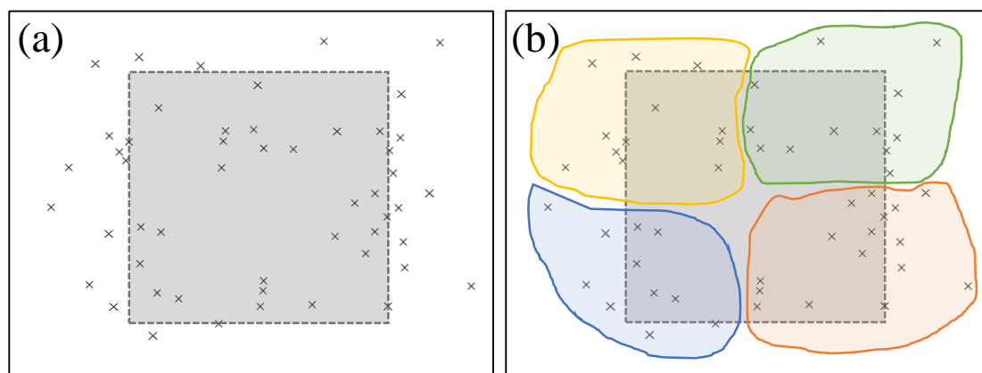
Figure 7. Human demonstrations and their clustered results. (a) Initial positions of the pegs (“x” symbols) with respect to the hole. The edge of the gray box indicates the boundary between the outside and inside of the hole. (b) Clustering results obtained by the k-means clustering algorithm using the reaction force/moment measured at the initial positions. We performed approximately 50 demonstrations to evaluate the clustering results.
