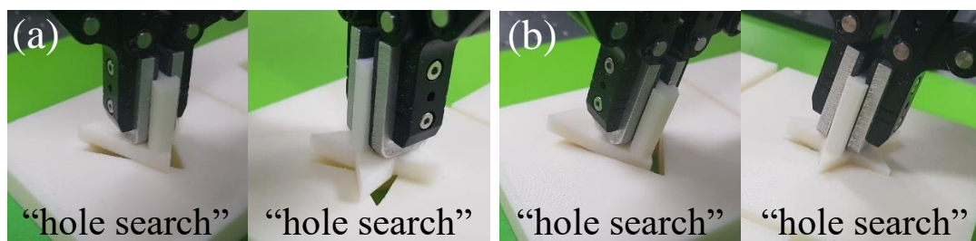
Figure 11. Using motor skills learned from rectangle shape for different shapes of triangle and star: (a) failure cases; and (b) the successful completion of the cases in (a).
