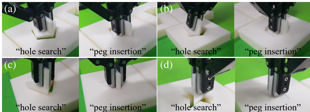
Figure 10. Using motor skills learned from the rectangle shape for different shapes: (a) pentagon; (b) hexagon; (c) triangle; and (d) star. These figures indicate the successful cases in which the motor skills learned for the rectangle shape can be used for other shapes without any generalization process.
