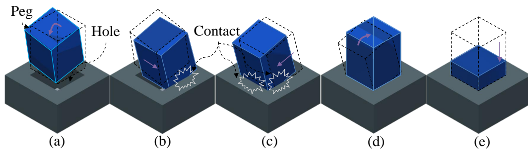
Figure 2. “Hole search” and “peg insertion” motions in the peg-in-hole task: (a) tilt-search motion; (b) single-point contact motion, which pushes on one face of the peg to make contact with the hole; (c) two-point contact motion, which pushes two faces of the peg to make contact with the hole; (d) tilting motion to align that the peg and hole; and (e) pushing motion to push the peg down into the hole.
