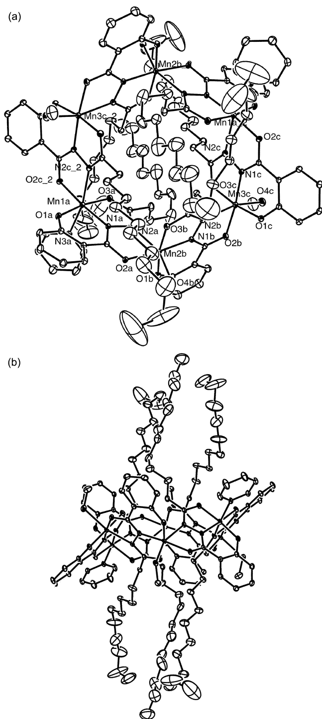
Figure 5. (a) An ORTEP drawing of complex 5 , Mn_6(lshz)_6-(MeOH)_4(py)_2 . As in complex 3 , complex 5 is in the crystallographic inversion center and A, B, and C in manganese ions could be related to each other using a pseudo- S_6 symmetry operation. The methanol is coordinated to the manganese B center and C center, the pyridine is coordinated to the manganese A center. Hydrogen atoms have been omitted for clarity. (b) Side view of complex 5 . The alternating side chains are aligned approximately at a right angle to the plane of the metallamacrocycle.
