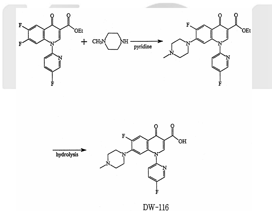
Fig. 1. Chemical structure of DW-116 and synthetic routines.
