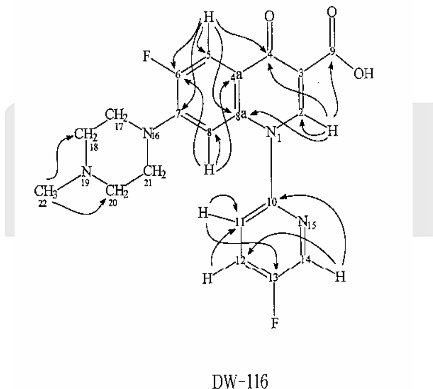
Fig. 2 Chemical structure of DW-116 with numbering scheme and selected 1 H- 13 C J-network connectivities
