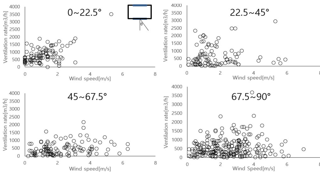
Figure 2. Ventilation rate according to wind speed considering wind direction.
