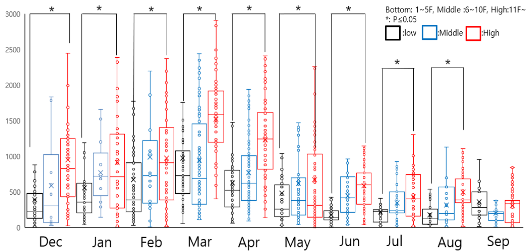
Figure 3. Monthly ventilation rate considering floor level
