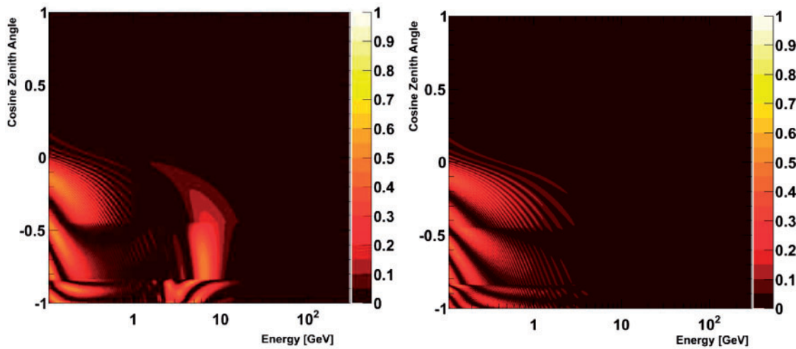
Fig. 35. Atmospheric neutrino oscillation probabilities as a function of energy and cosine of the neutrino zenith angle ( -1 corresponds to upward-going). The left (right) plot shows the \nu_\mu \rightarrow \nu_e ( \bar{\nu}_\mu \rightarrow \bar{\nu}_e ) probability. In this plot the normal mass hierarchy is assumed. For an inverted hierarchy the features in the neutrino plot move to the antineutrino plot and vice versa.
