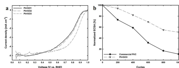
Fig. 3. ORR activities of the prepared Pt/rGOs (a) and normalized ECSA values of the Pt/rGO3 and commercial Pt/C throughout the ADT.
