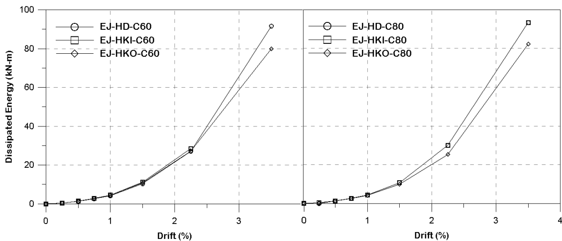
Fig. 8 Energy dissipation capacities of test specimens
