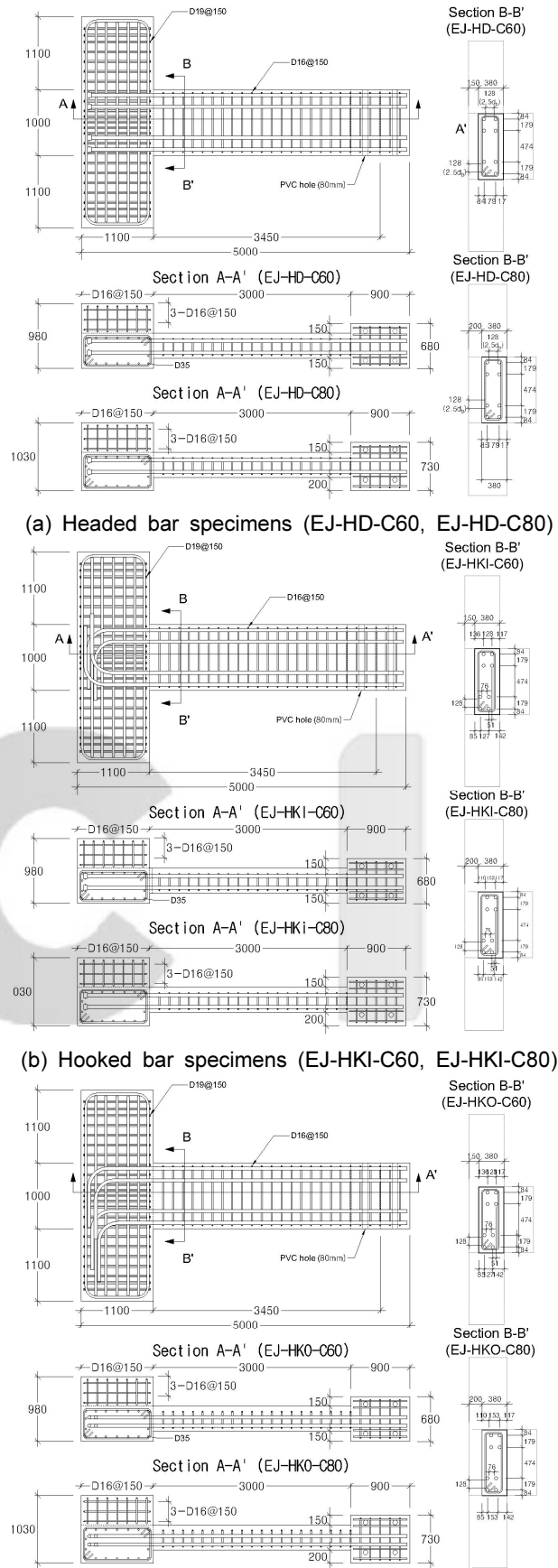
(c) Hooked bar specimens (EJ-HKO-C60, EJ80-HKO-C80)
