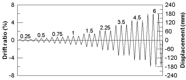
Fig. 3 Cyclic loading history
