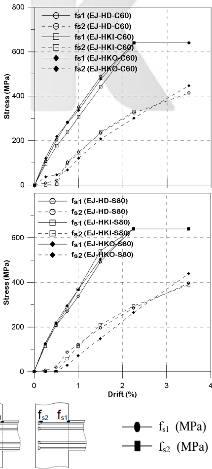
Fig. 6 Bar tensile stresses (EJ measured)
