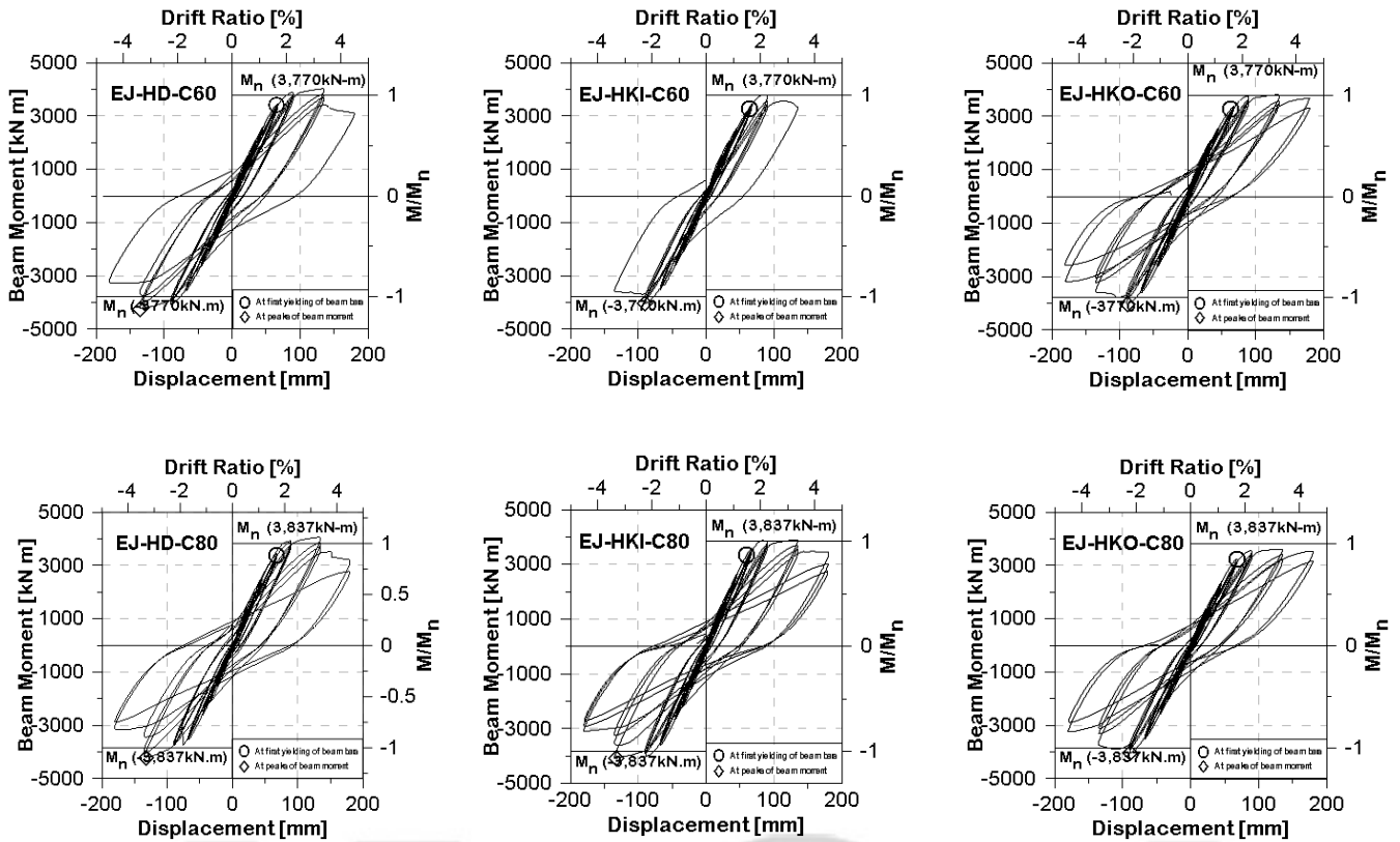
Fig. 5 Beam moment versus drift ratio relations
