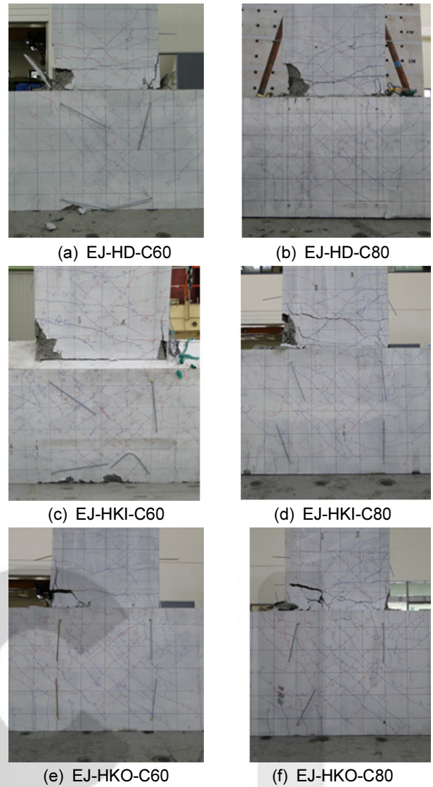
Fig. 4 Test failure mode
