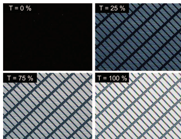
Fig. 2 Microscopic textures of the VAC LCD at various gray levels. (Color online only.)
