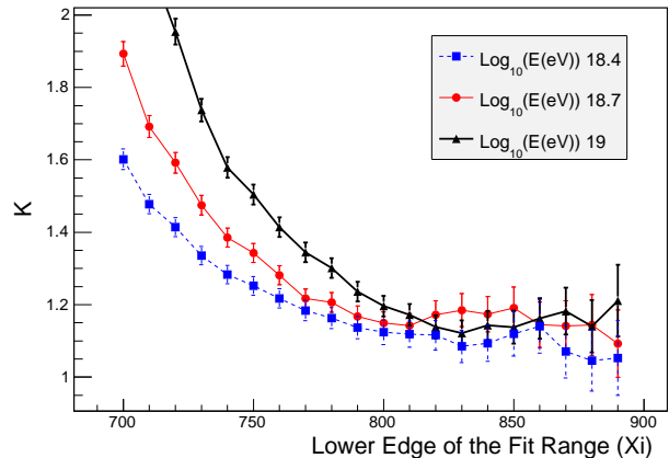
FIG. 2. The value of K vs. the lower edge in the fit range X_i to the tail of the X_{max} distribution for several data sets 10^{18.4} , 10^{18.7} , and 10^{19} eV simulated using CONEX with the high energy model QGSJETII.4. Each data set contains 10,000 simulated events.
