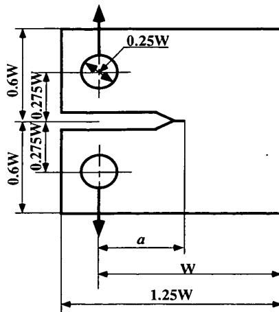
Fig. 3 Compact tension (CT) specimen of bulk epoxy resin. ( W = 24\text{mm} , a/W \cong 0.5 , Thickness = 8\text{mm} )
