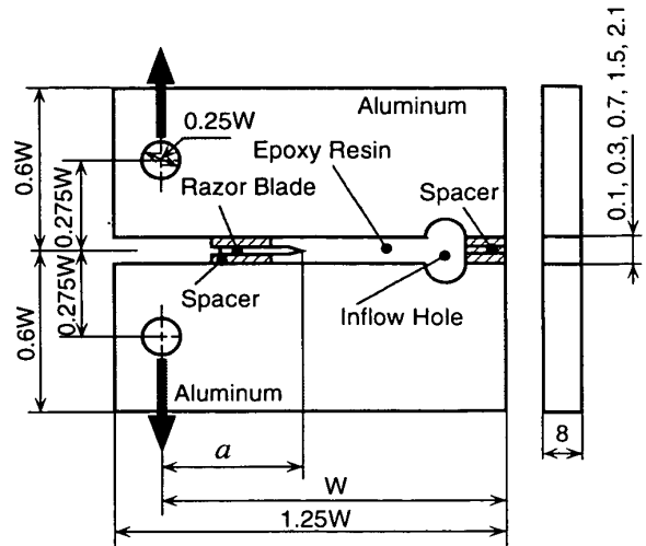
Fig.2 Compact tension (CT) adhesive joint specimen (W = 48mm, a/W ≐ 0.5)
