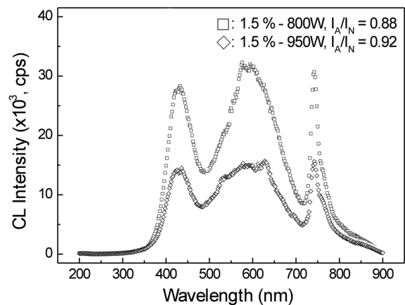
Fig. 4. The effect of microwave power (800 W and 950 W) on the CL spectra ( N_2/(CH_4+H_2)=1.5\% ).
