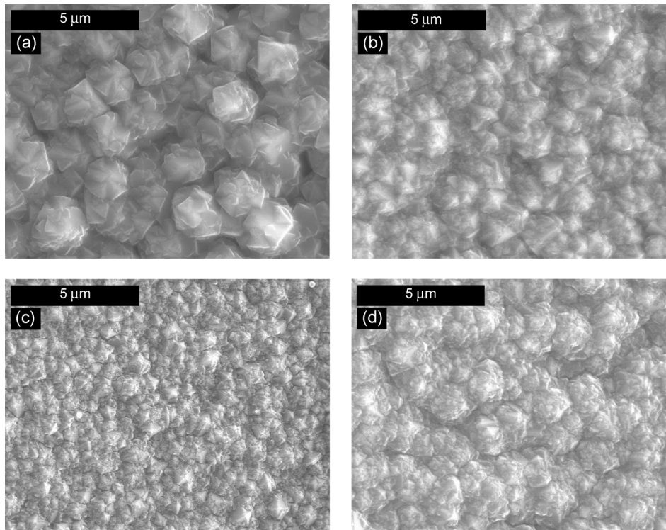
Fig. 1. The FE-SEM images of diamond films grown at 800 W; (a) N_2/(CH_4+H_2)=0\% , (b) N_2/(CH_4+H_2)=0.5\% , (c) N_2/(CH_4+H_2)=1.5\% , (d) N_2/(CH_4+H_2)=2.0\% .
