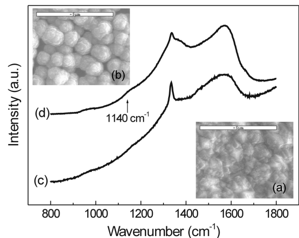
Fig. 5. The FE-SEM images ((a) and (b)) and Raman spectra ((c) and (d)) of nitrogen-incorporated diamond films grown at N_2/(CH_4+H_2)=0.5\% and 800 W; (a) and (c) without oxygen, (b) and (d) with oxygen ( O_2/(CH_4+H_2)=0.5\% ).
